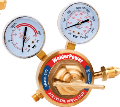
Acetylene Regulator SR450-300
